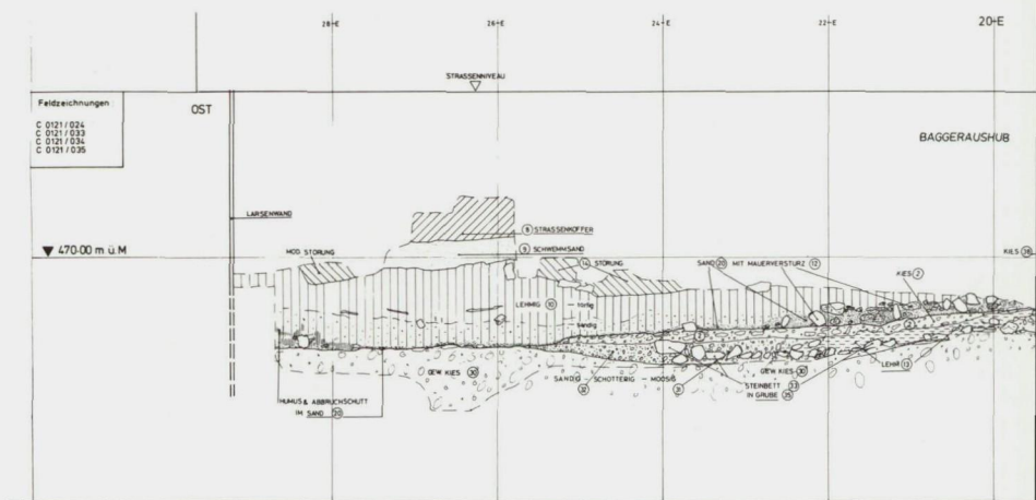
Abb. 3: Plan D 0121/002, M 1:100
