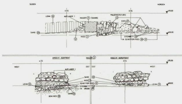
Abb. 2: Plan D 0121/003, M 1:100
